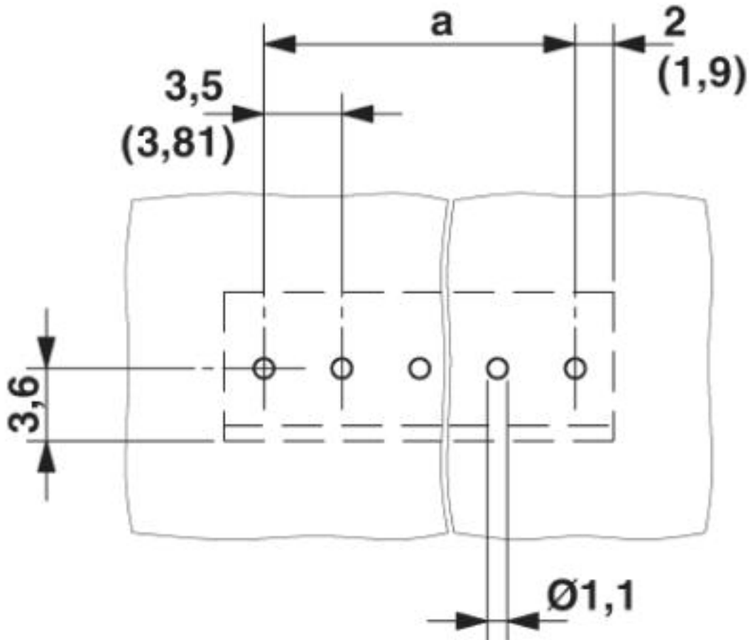
Drilling diagram
